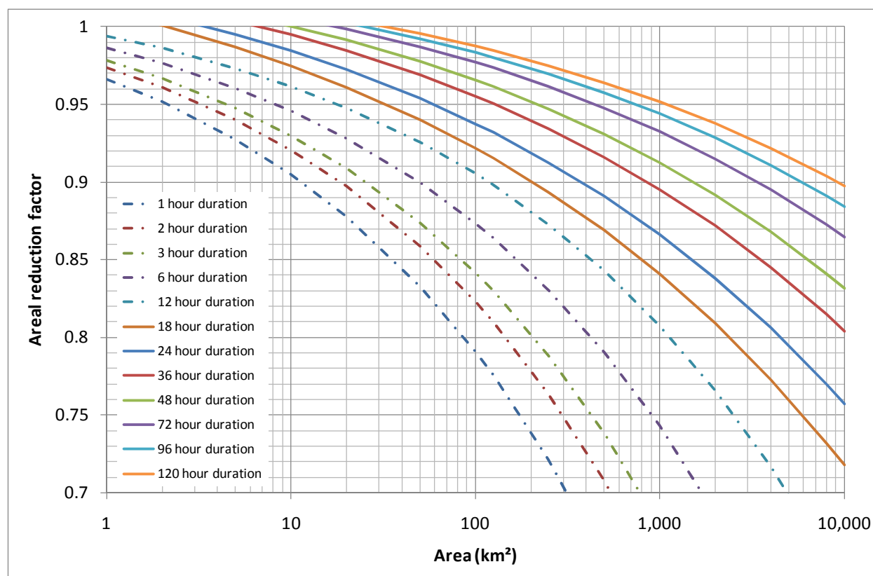
Figure 4-12 ARF in the NSW GSAM (including the ACT) region for AEP = 0.5 for varying rainfall durations
