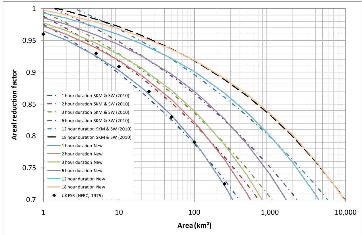
Figure A- 5 Revised short duration ARF curves derived for the GTSM-R region of NSW, compared to the 18 hour duration ARF curve for the GTSM-R region of NSW from Sinclair Knight Merz and State Water (2010), the 1 hour ARF values from Natural Environmental Research Council (1975) and the interim short duration ARF curves derived for the GTSM-R region of NSW by Sinclair Knight Merz and State Water (2010)
