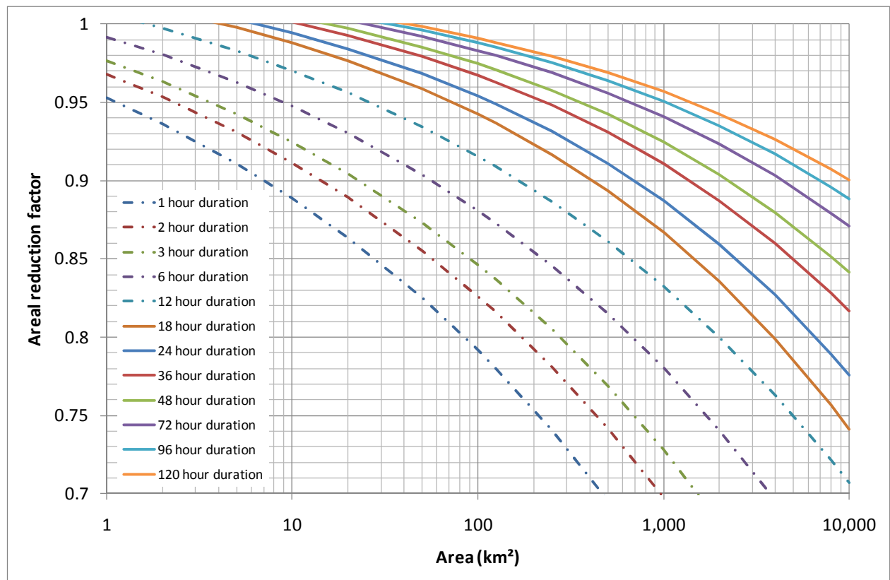
Figure 4-3 ARF for South Australia for AEP = 0.5 for varying rainfall durations
