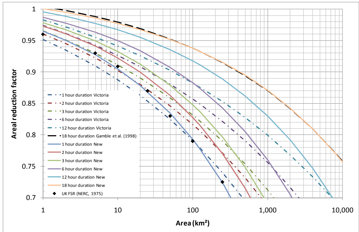
Figure A- 6 Revised short duration ARF curves derived for Tasmania, compared to the 18 hour duration ARF curve for Tasmania from Gamble et al. (1998), the 1 hour ARF values from Natural Environmental Research Council (1975) and the interim short duration ARF curves from Siriwardena and Weinmann (1996a) that had previously been recommended for use in Tasmania by Gamble et al. (1998)
