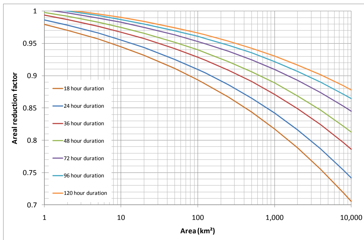
Figure 4-7 Summer ARF for the rest of Western Australia for AEP = 0.5 for varying rainfall durations
