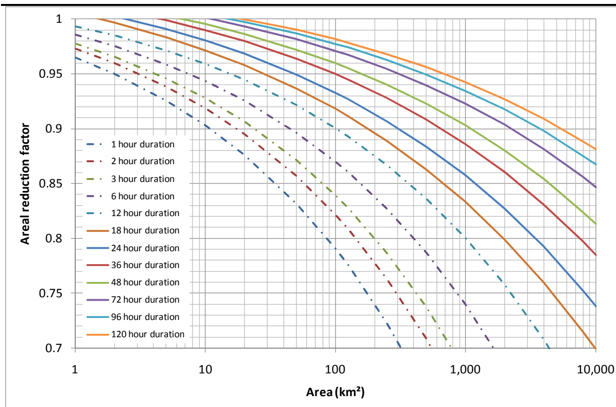
Figure 4-11 ARF in the NSW GTSM-R region for AEP = 0.5 for varying rainfall durations
