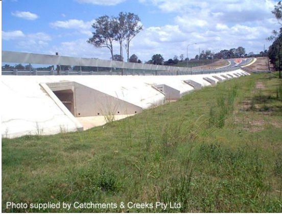
Photo 28: Series of floodplain culverts
