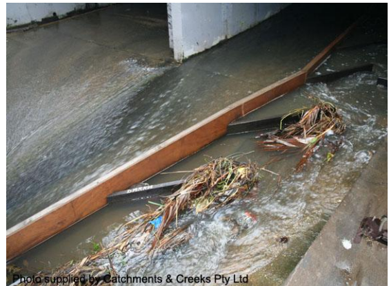
Photo 13: Debris can be trapped by fish passage baffles
